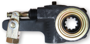
GUNITE Clearance Sensing Collar Lock Clevis
